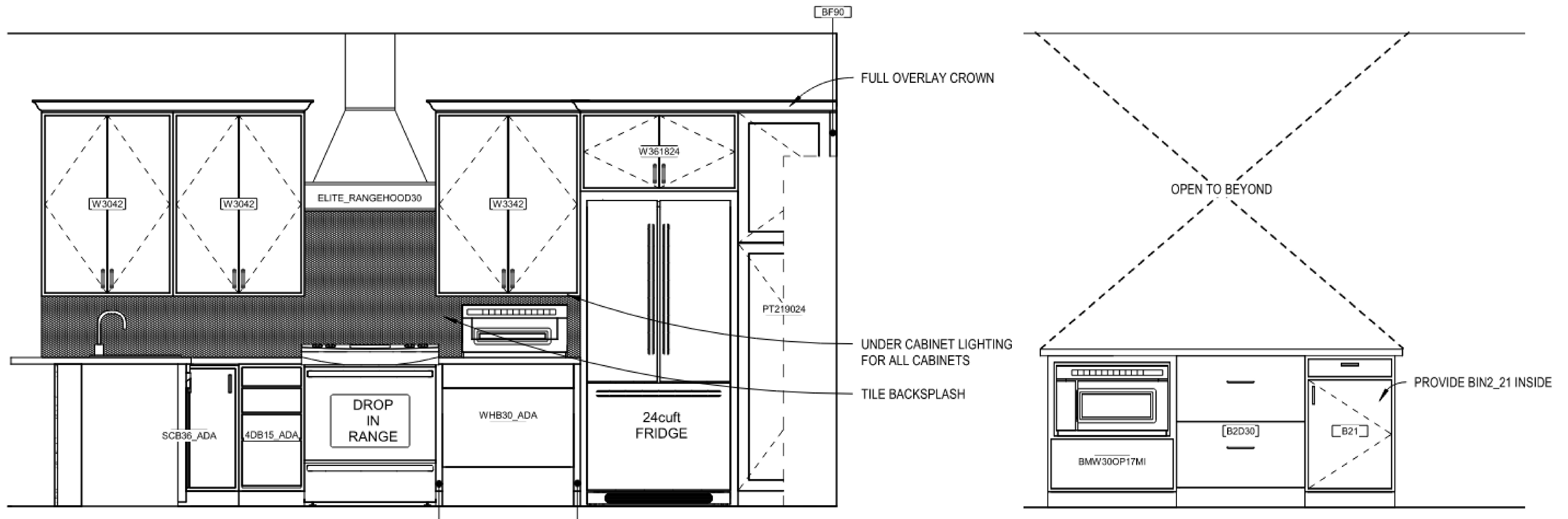
Kitchen Elevations
